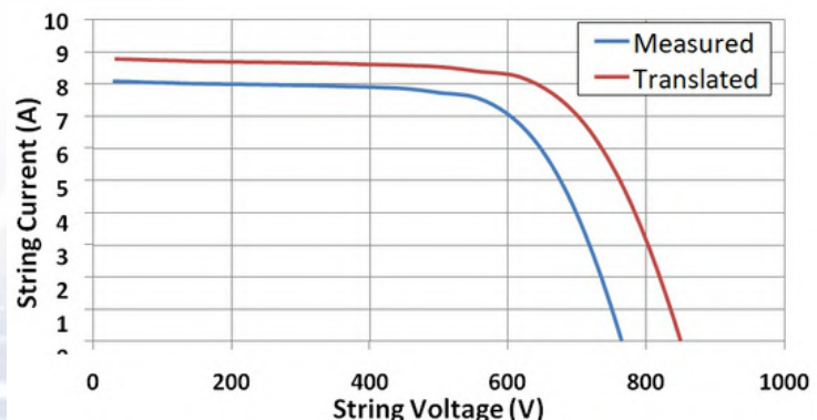
IV Curve Tracer
