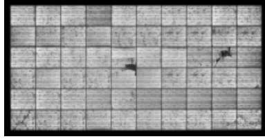
Portable EL Inspection System
