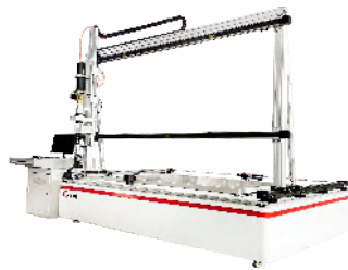
Hail Impact Testing Machine IEC61215, IEC61646, UL1703
